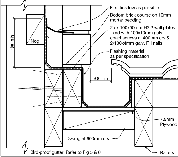
FIG.1 WALL AT SIDE OF ROOF SLOPE Option: Secret Gutter - Timber Support
