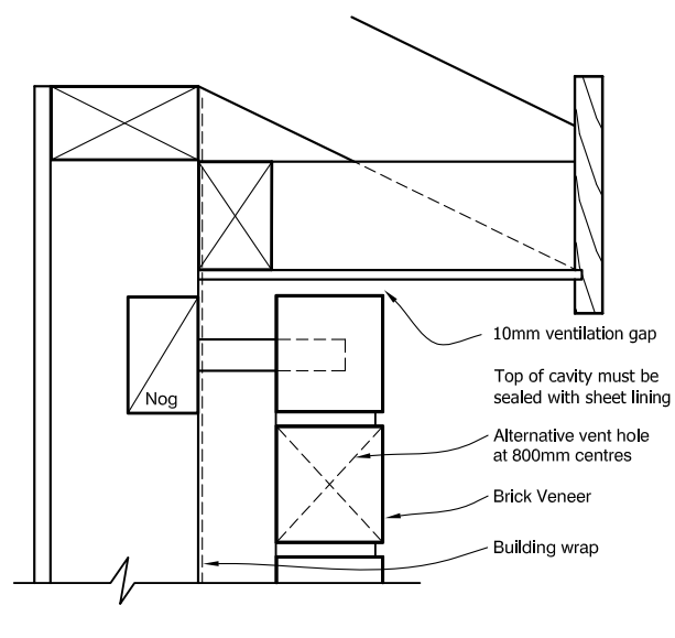
FIG.18 FLAT SOFFIT
